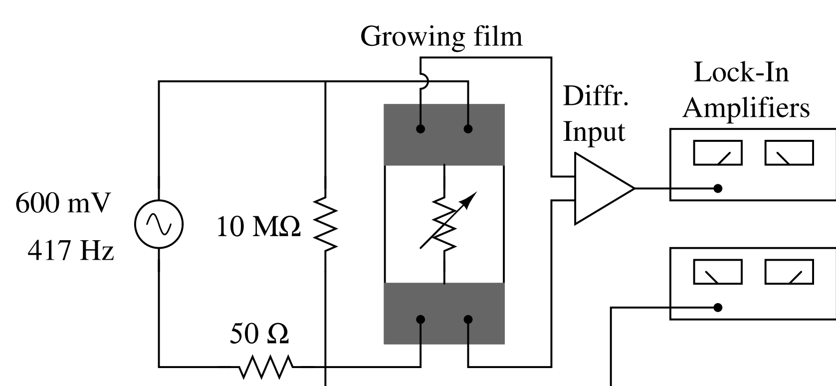
Figure 2: A schematic drawing of the in-situ measuring circuit.
