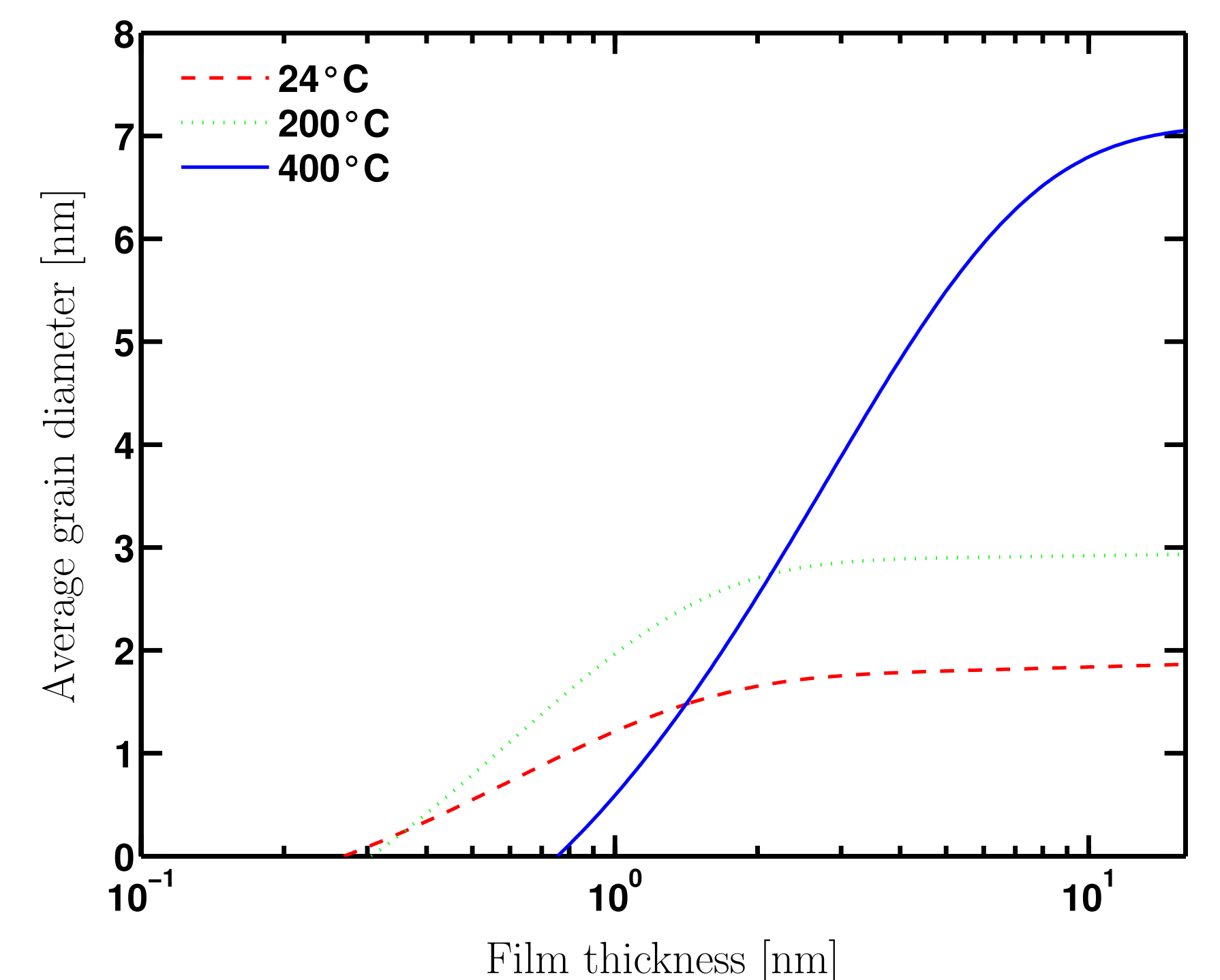
Figure 5: The grain size models used to fit the resistivity of the films in Fig. 4 to the combined F-S and M-S model.
